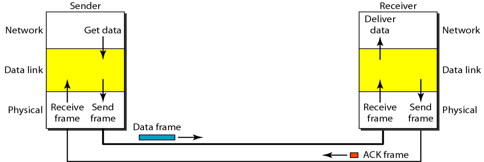
Figure 11.8 Design of Stop-and-Wait Protocol
