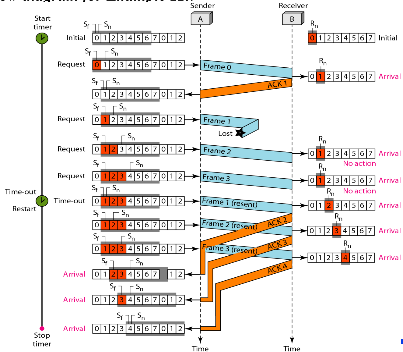
Figure 11.17 Flow diagram for Example 11.7
